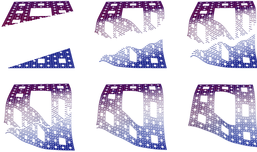
FIGURE 2. Nonlocal diffusion on the Sierpinski carpet. Solution with J(x, y) = 100e^{-100|x-y|^2} and f(x) = \mathbb{I}_{\{x_2 > x_1/2\}}(x) . Snapshot of solution, from left to right and top to bottom, at t = 0, 0.5, 1, 2, 4, 8 . The space X is decomposed into 8^4 components X_k . Each set X_k = \phi_k(X) was drawn as \phi_k(S) with S the unit square. The time discretization was done with the fourth order Runge-Kutta scheme using \Delta t = 0.05 .
